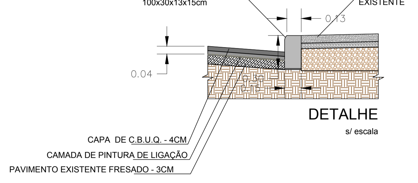
MEIO-FIO DE CONCRETO 100x30x13x15cm
